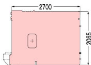
OUTLINE unit:mm M/C HEIGHT(FL.):2980
